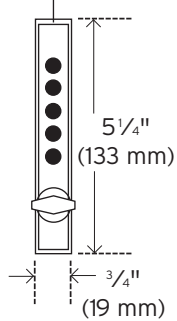
Escutcheon Plate
